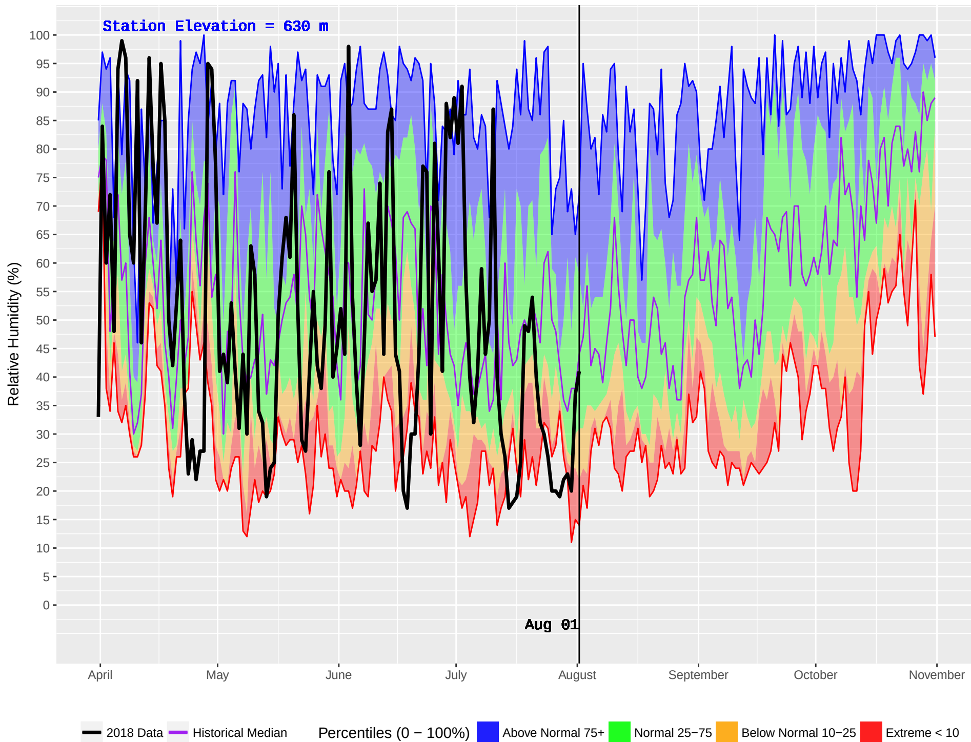
ANDERSON CREEK (977) : Historical (2007–2016) and Current (2018) Daily Relative Humidity
